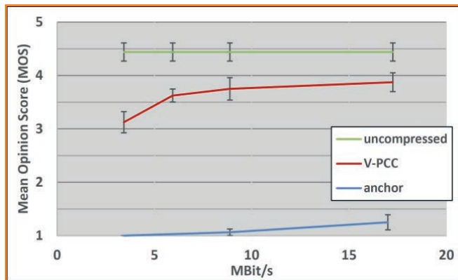
Figure 5: Subjective evaluation results for sequences RedandBlack and Longdress (2).
