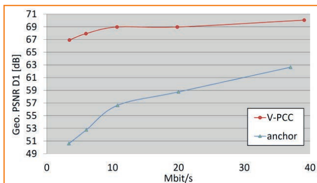
Figure 6: Objective geometry and texture RD-curves for sequence Soldier (2).
