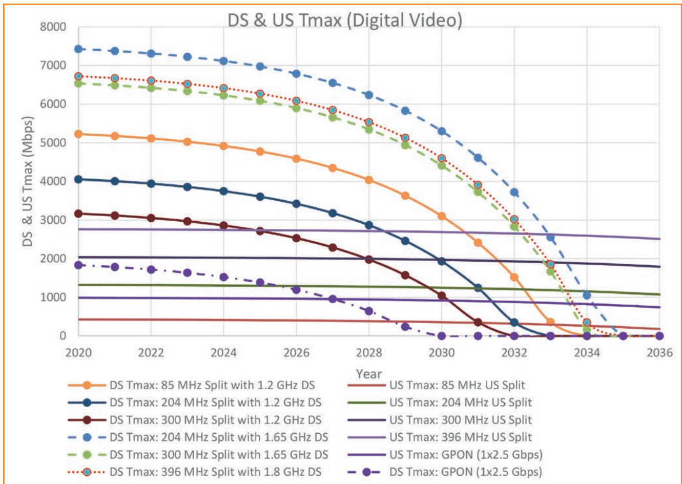
Figure 6: US & DS Tmax values that can be offered over time for various split options and DS spectrum sizes (SG size = 64, 66 Digital video channels)
