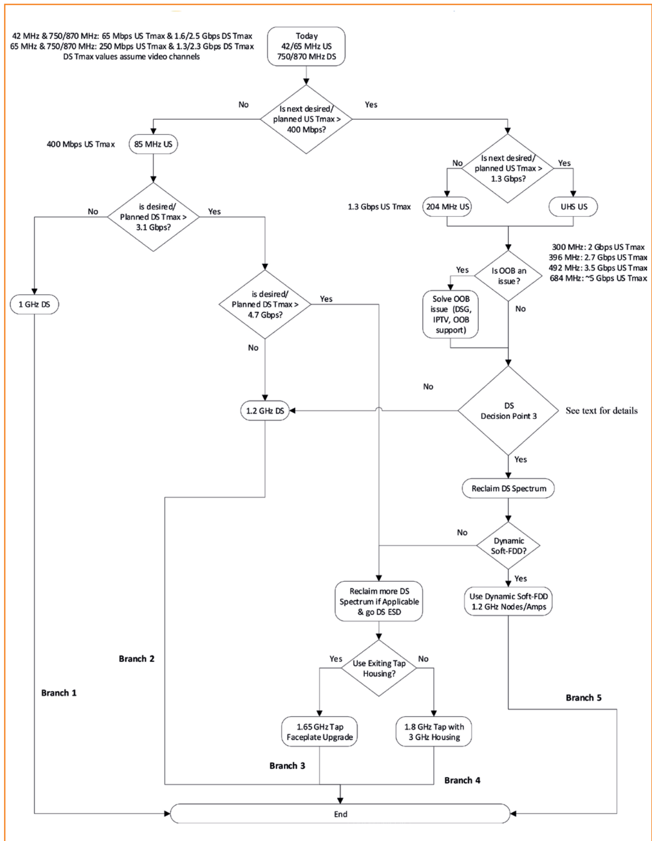
Figure 3: Decision tree combining multiple inter-related network migration tools: traditional FDD with DOCSIS 3.0 splits, DOCSIS 3.1/ DOCSIS4.0 split change, Dynamic Soft-FDD and ESD
