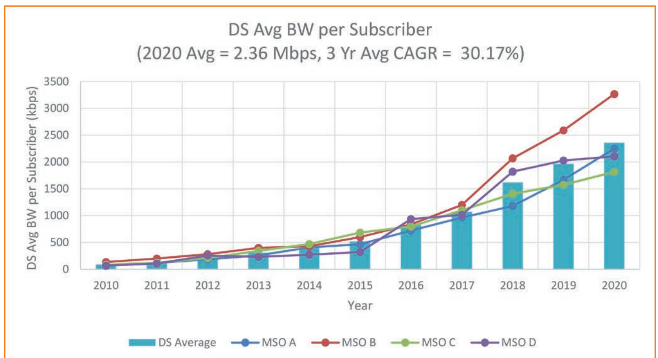
Figure 1: DS Tavg latest statistics before COVID-19
