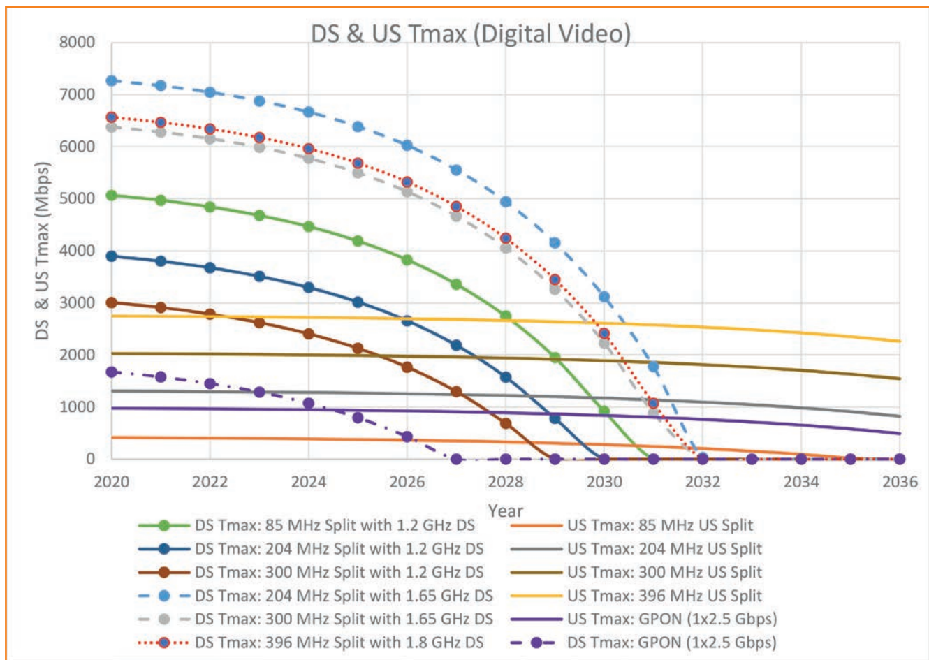
Figure 5: US & DS Tmax values that can be offered over time for various split options and DS spectrum sizes (SG size = 125, 66 Digital video channels)
