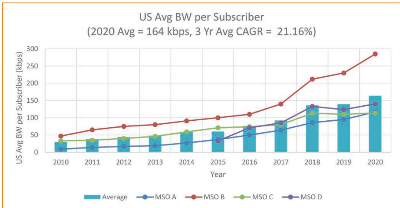
Figure 2: US Tavg latest statistics before COVID-19
