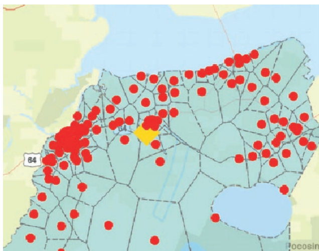
Figure 3: FWA topology map of Washington County
