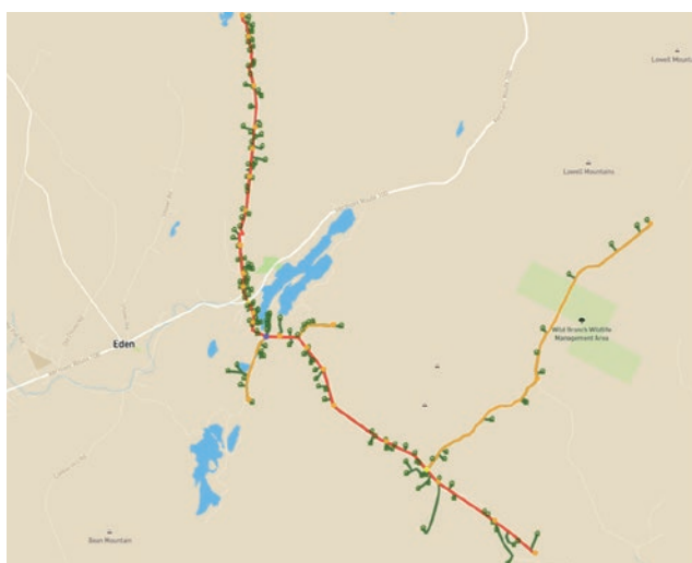
Figure 5: LLD Eden Mills, Vermont (courtesy of Vetro). 6
