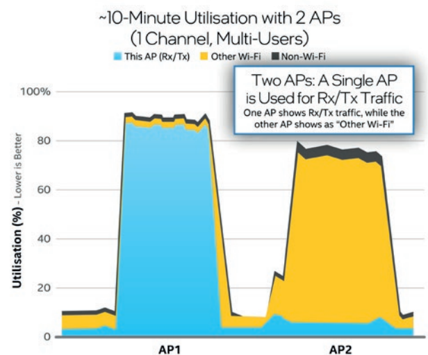
Figure 5: Two neighbouring APs operating on the same channel have the same utilisation; however, only one AP has users connected and is generating data.
