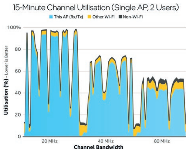
Figure 3: Wi-Fi 6 testing with two users per AP showed that we could increase bandwidth and decrease air utilisation without penalty.
