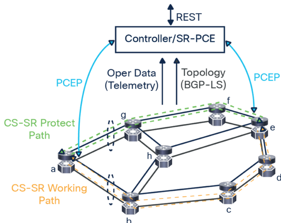
Figure 5: Circuit-Style Segment Routing - Routed Optical Networking innovation that enables transport friendly provisioning of protected services.
