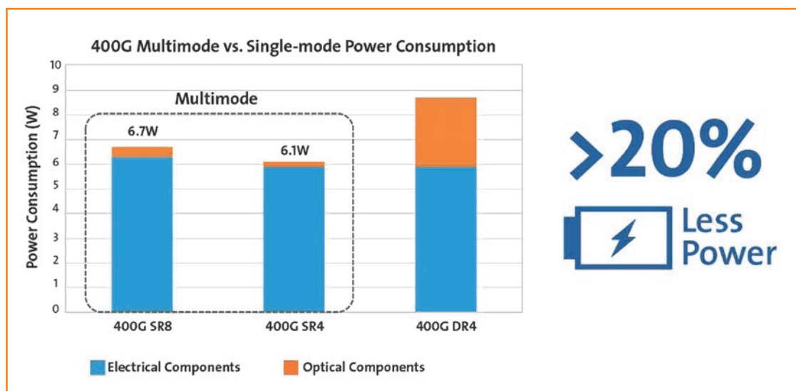
Figure 4. Multimode vs. Single-mode 400G Transceiver Power Consumption Comparison
