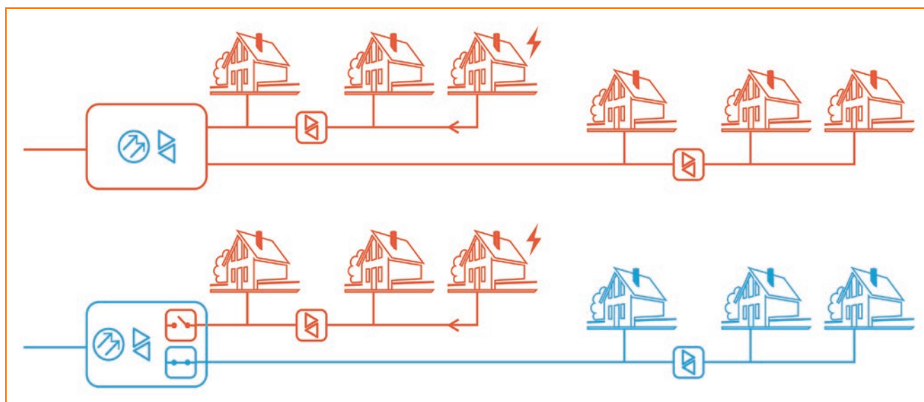
The failing segments can be segregated with ingress switches.
